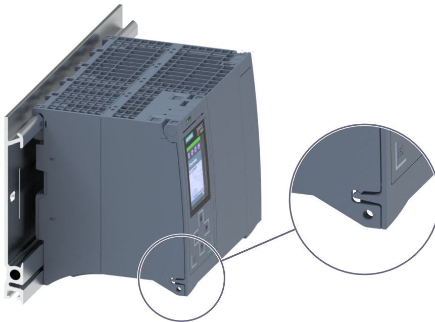
Figure 3-3 Locking latch on the CPU
