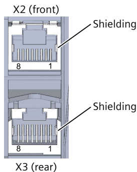
Figure 4-1 Interfaces X2 and X3
