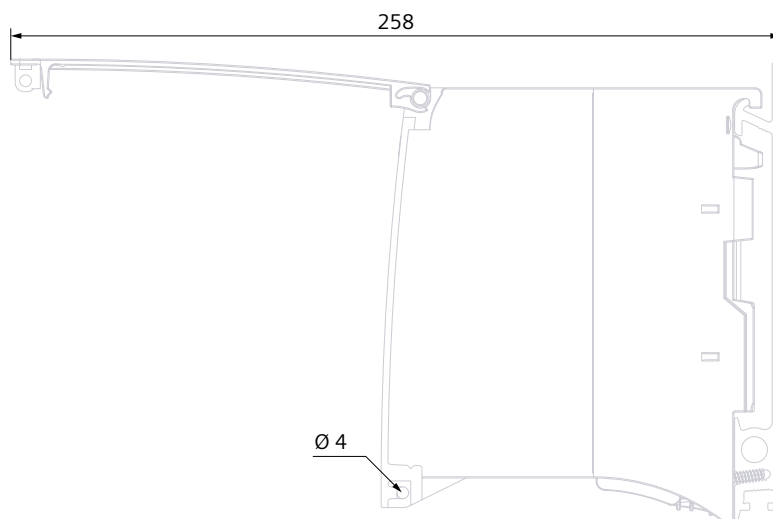
Figure A-2 Dimensional drawing CPU 1518-4 PN/DP, side view with open front panel
