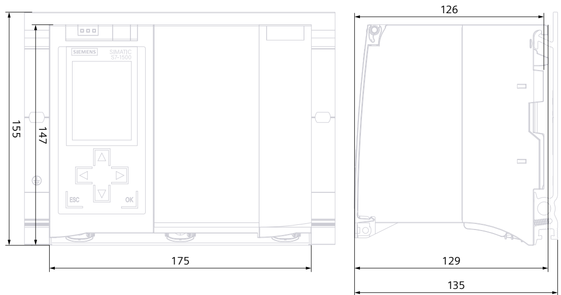
Figure A-1 Dimension drawing of the CPU 1517T-3 PN/DP, front and side view
