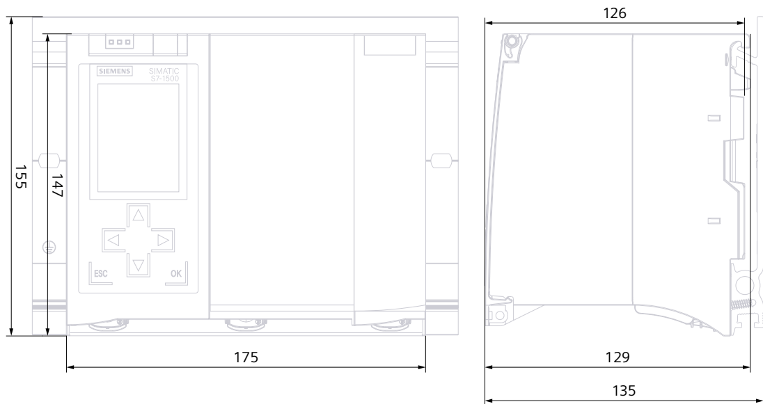
Figure A-1 Dimension drawing of CPU 1517-3 PN/DP, front and side views
