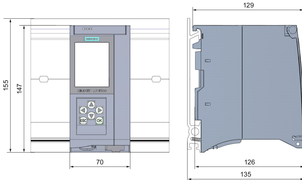
Figure A-1 Dimensional drawing of the CPU 1515T-2 PN
