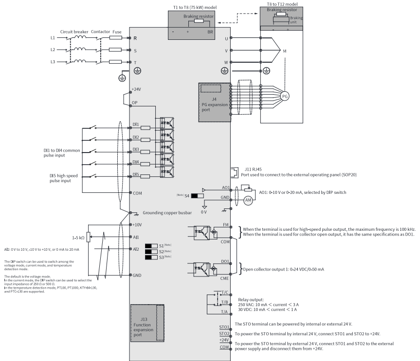
Figure 2-1 Standard wiring
