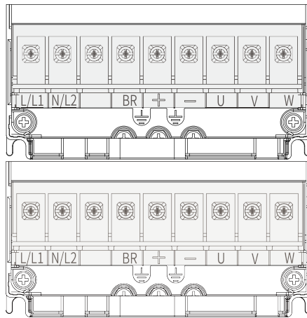
Figure 2-3 Main circuit terminals of T2 models (single phase)
