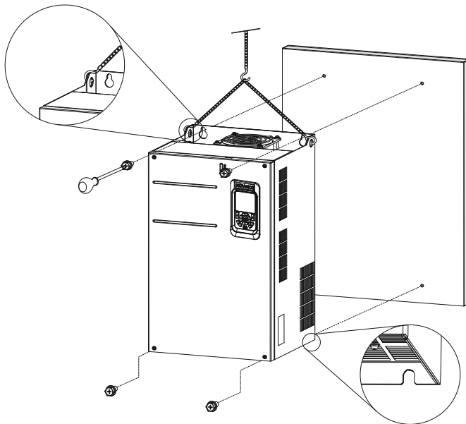
Figure 1-5 Backplate mounting (T7 to T9 models)
