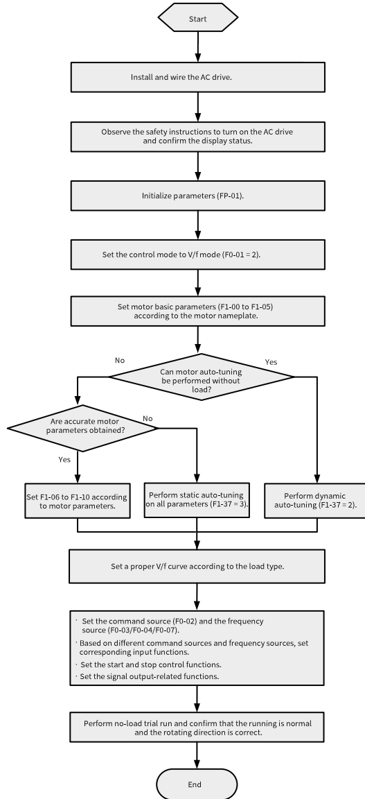
Figure 3-3 Commissioning process in V/f control mode
