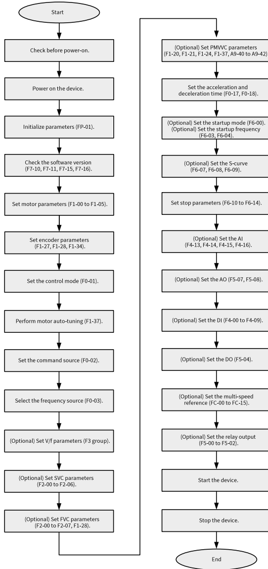
Figure 3-2 Commissioning process
