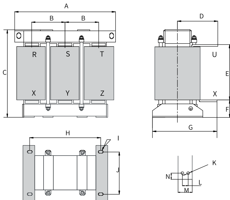
Figure 5-22 Dimensions of 800 A/1000 A AC input reactors
