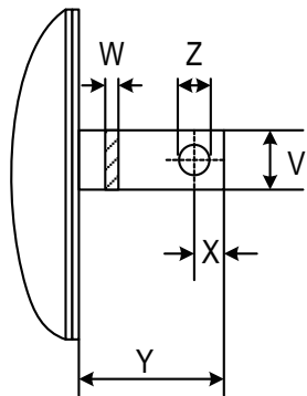
Figure 5-26 Dimensions of copper busbars
