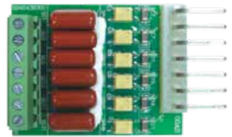
▪ EME-D611B Multi-function Input Terminal MI1~MI6-COM Card (For External Installation)
